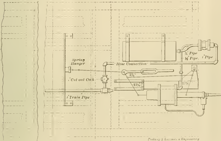
PLAIN VIEW OF DIVIDED OR TWIN BRAKE.
